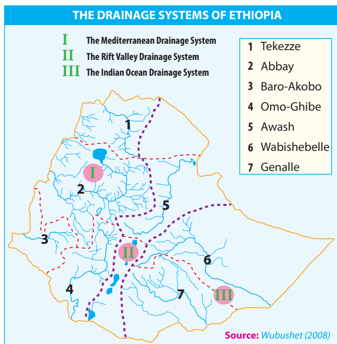
Figure 3.9: Drainage Systems of Ethiopia
