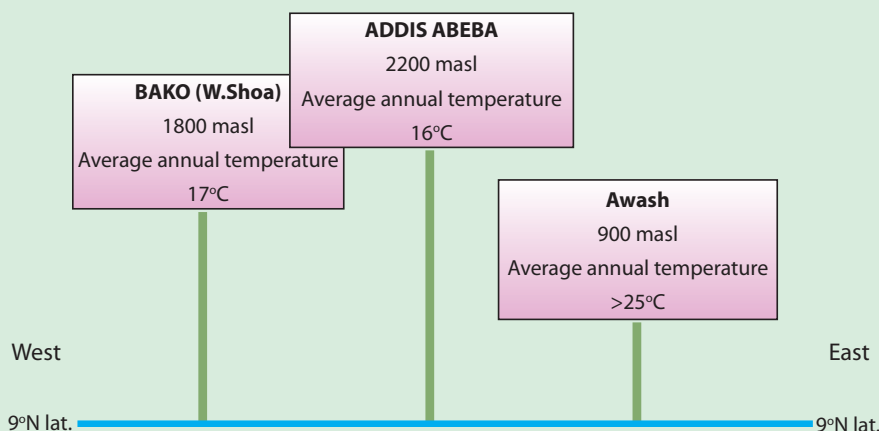
Figure 3.11: The role of altitude in modifying temperatures
