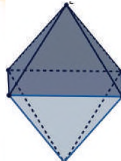
Octaedro
