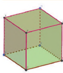
Hexaedro
